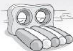
Game 1
